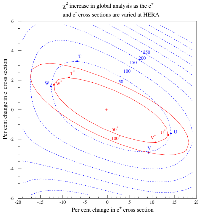
Fig. 5. \Delta\chi^2 = 50, 100, \dots contours, where \Delta\chi^2 is the increase in \chi^2 from the global MRST2001 minimum, obtained by performing new global fits with F_2^{CC}(e^\pm p) fixed at values in the neighbourhood of their value in unconstrained MRST2001 fit. The \Delta\chi^2 = 50 contour is taken to represent the errors on F_2^{CC}(e^\pm p) (arising from the experimental errors on the data used in the global fit). The extrema sets of partons (T,U,...) are discussed in the text. The dashed contours are obtained if \alpha_S(M_Z^2) is allowed to vary. The superimposed solid \Delta\chi^2 = 50, 100 contours are obtained if \alpha_S(M_Z^2) is fixed at 0.119
