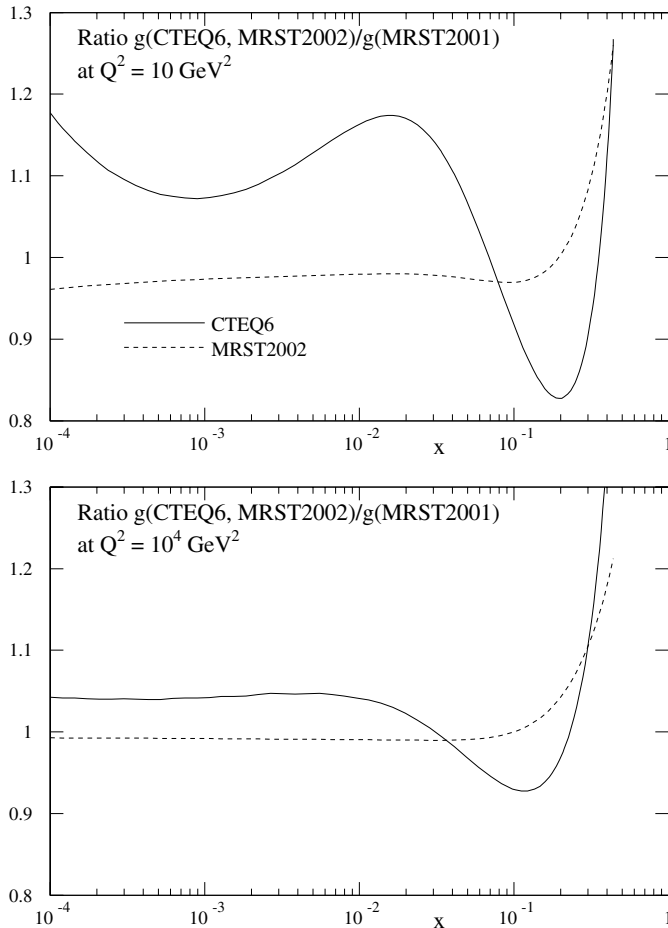
Fig. 14. The CTEQ6 [5] and MRST2002 gluon compared to MRST2001 [9] gluon at Q^2 = 10 and 10^4 \text{GeV}^2
