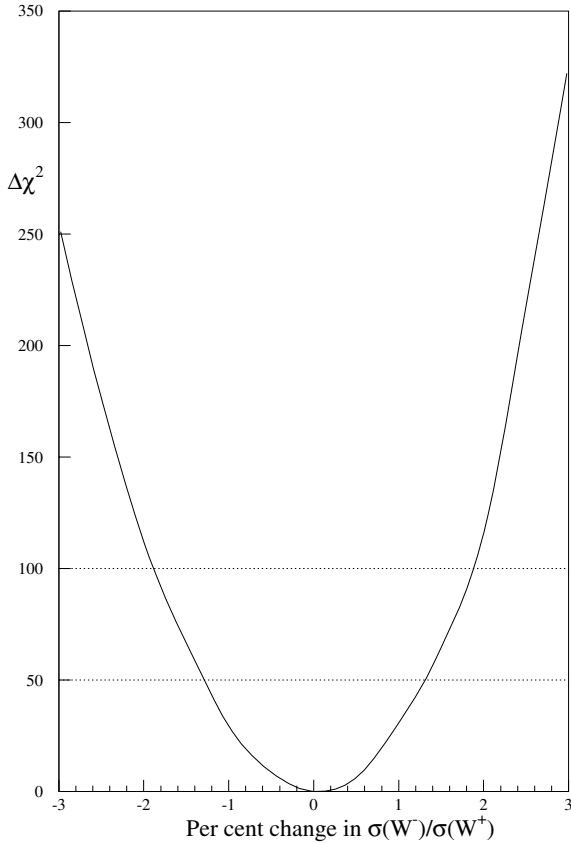
Fig. 12. The variation of \chi^2 obtained by performing global fits with \sigma(W^-)/\sigma(W^+) fixed at different values in the neighbourhood of the value obtained in the unconstrained MRST2001 fit. For \Delta\chi^2 = 50 we see that the uncertainty in the ratio is \pm 1.3\%
