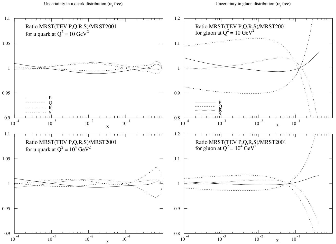
Fig. 11. As for Fig. 10 but with \alpha_S(M_Z^2) allowed to vary
