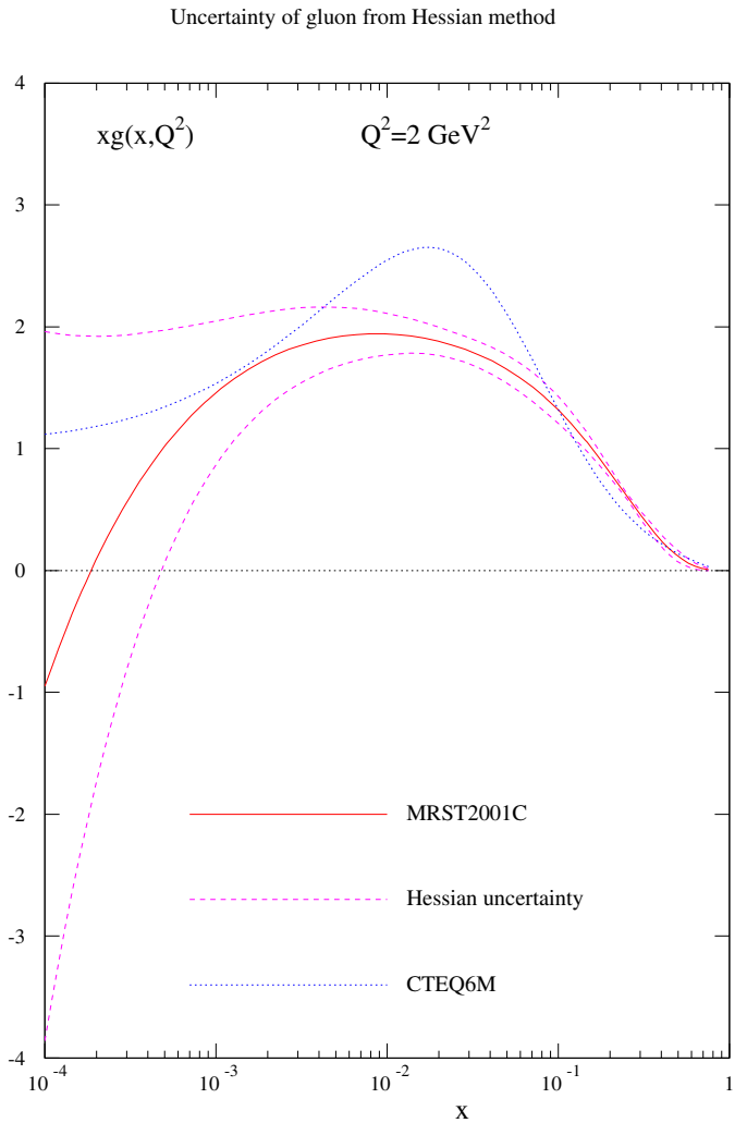
Fig. 4. The uncertainty on g(x, Q^2) at Q^2 = 2 \text{ GeV}^2 obtained using the Hessian approach with \Delta\chi^2 = 50 . Also shown is the CTEQ6M distribution
