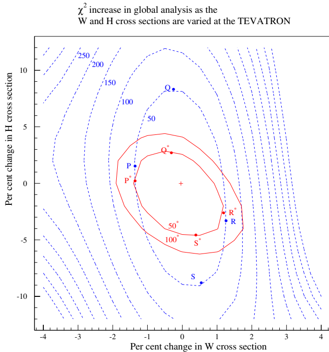
Fig. 9. As for Fig.7, but for the Tevatron energy of \sqrt{s} = 1.8 TeV
