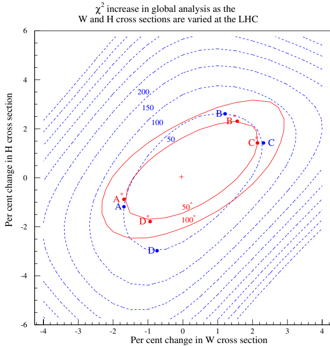
Fig. 7. Contours with \Delta\chi^2 = 50, 100 \dots obtained by performing global fits with the values of \sigma_W and \sigma_H , at the LHC energy, fixed in the neighbourhood of their values predicted by the unconstrained MRST2001 fit. The \Delta\chi^2 = 50 contour is taken to represent the errors on \sigma_W and \sigma_H (arising from the experimental errors on the data used in the global fit). The extrema sets of partons (A,B,...) are discussed in the text. The dashed contours are obtained if \alpha_S(M_Z^2) is allowed to vary. The superimposed solid \Delta\chi^2 = 50, 100 contours are obtained if \alpha_S(M_Z^2) is fixed at 0.119
