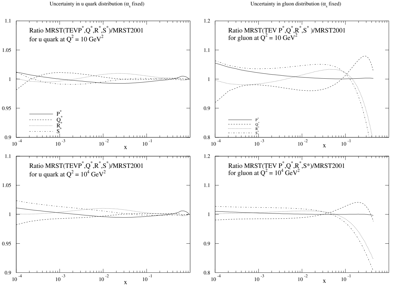
Fig. 10. The up quark and gluon distributions at Q^2 = 10 and 10^4 \text{GeV}^2 found in the extrema global fits on the \Delta\chi^2 = 50 contour of the \sigma_{W,H} (Tevatron) plot of Fig. 9 with \alpha_S(M_Z^2) fixed at 0.119
