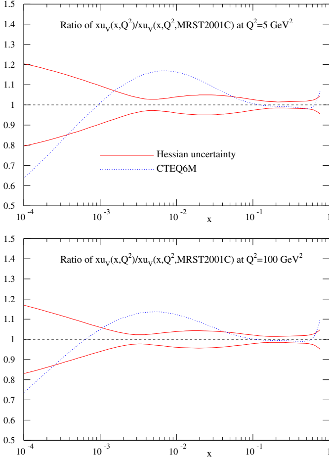
Fig. 1. The uncertainty on u_V(x, Q^2) at Q^2 = 5 \text{ GeV}^2 and 100 \text{ GeV}^2 obtained using the Hessian approach with \Delta\chi^2 = 50 . Also shown is the CTEQ6M distribution. The uncertainties are shown relative to the MRST2001 set of partons [9]; the label C is explained in footnote 4
