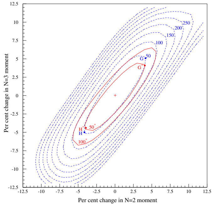
Fig. 13. The \Delta\chi^2 contours obtained by performing global fits with the values of the N = 2 and N = 3 moments of the u-d distribution fixed in the neighbourhood of their values predicted by the MRST2001 global fit. The dashed and solid curves correspond to fits with \alpha_S(M_Z^2) varying and fixed respectively
