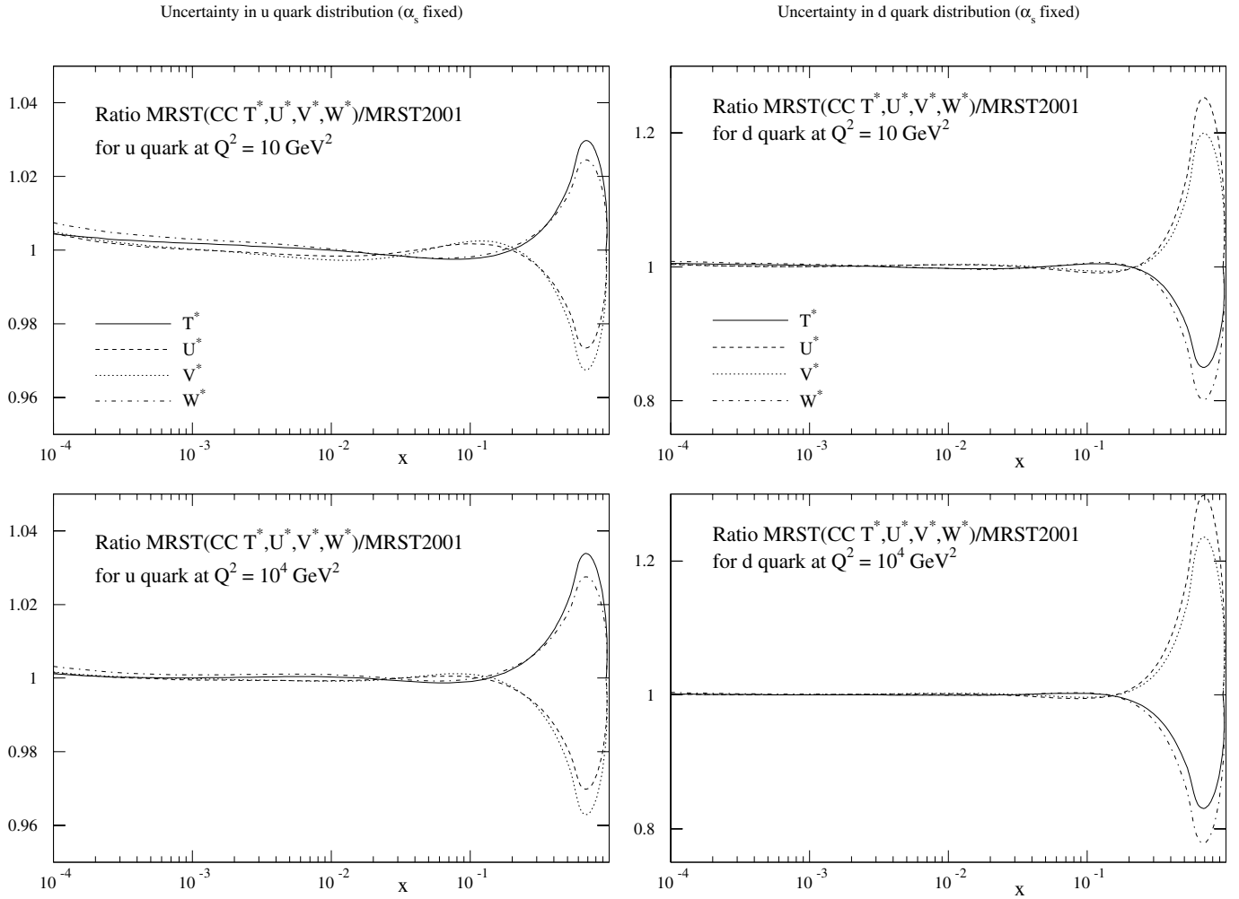
Fig. 6. The u and d quark distributions (at Q^2 = 10 and 10^4 \text{ GeV}^2 ) of the extrema fits which lie on the \Delta\chi^2 = 50 contour of Fig. 5 for fixed \alpha_S(M_Z^2) = 0.119
