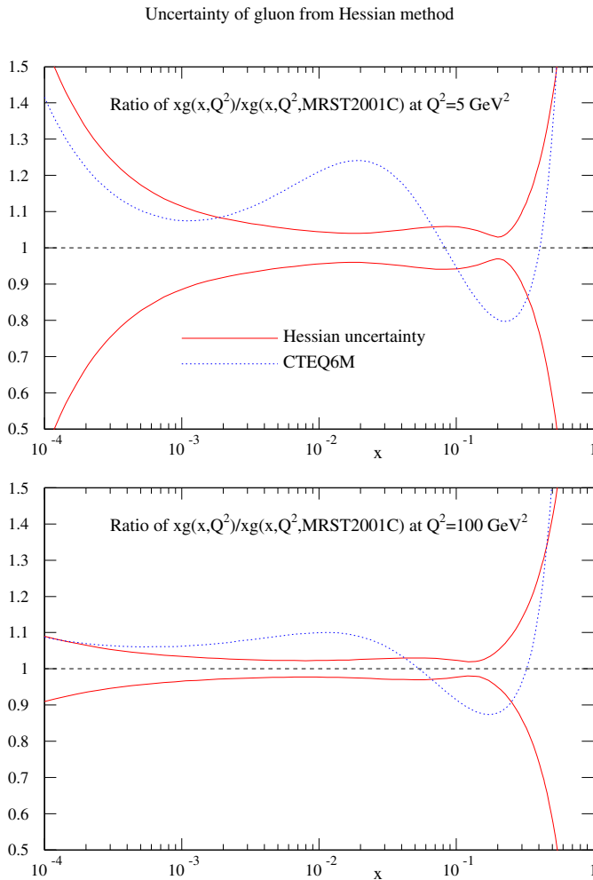
Fig. 3. The uncertainty on g(x, Q^2) at Q^2 = 5 \text{ GeV}^2 and 100 \text{ GeV}^2 obtained using the Hessian approach with \Delta\chi^2 = 50 . Also shown is the CTEQ6M distribution. The uncertainties are shown relative to the MRST2001 set of partons [9]; the label C is explained in footnote 4
