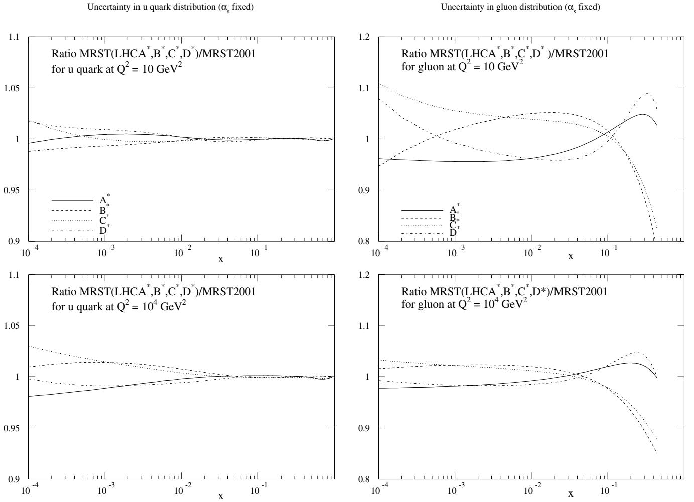
Fig. 8. The up quark and gluon distributions at Q^2 = 10 and 10^4 \text{GeV}^2 in the extrema global fits on the \Delta\chi^2 = 50 contour of the \sigma_{W,H}(\text{LHC}) plot of Fig. 7 for \alpha_S(M_Z^2) fixed at 0.119
