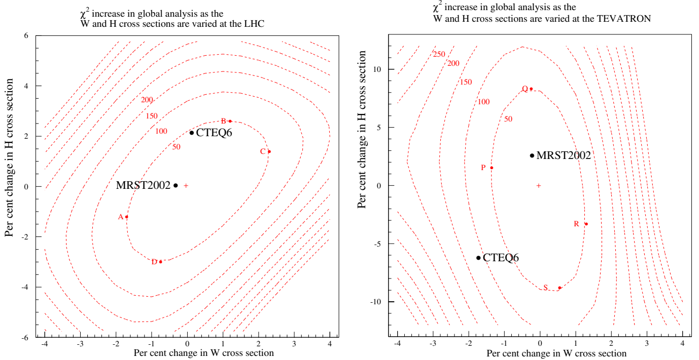
Fig. 15. The CTEQ6 [5] and MRST2002 predictions of \sigma_W , \sigma_H at the LHC and Tevatron energies, shown on the \Delta\chi^2 contour plots centered on the MRST2001 partons [9]. The \Delta\chi^2 contours are taken from Figs. 7 and 9 respectively, for the case in which \alpha_S(M_Z^2) is a free parameter. The inner contour with \Delta\chi^2 = 50 is taken to represent the error on the observables \sigma_W and \sigma_H arising from the experimental errors of the data that are used in the global fit
